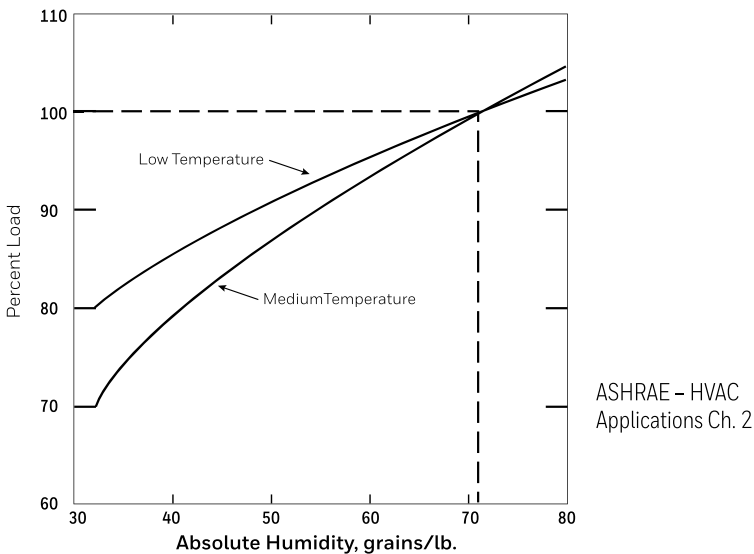
Figure 1. Refrigerated case load variation with store air humidity
